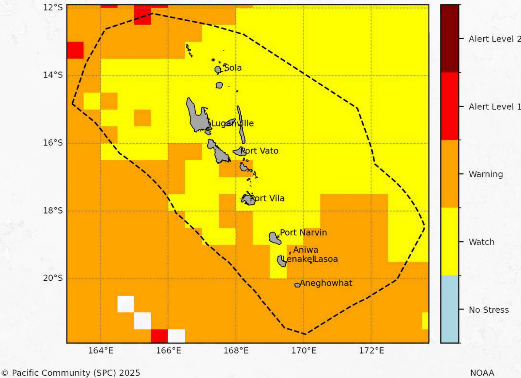
Vanuatu 4 Week Coral Bleaching Outlook: 9 February 2026
